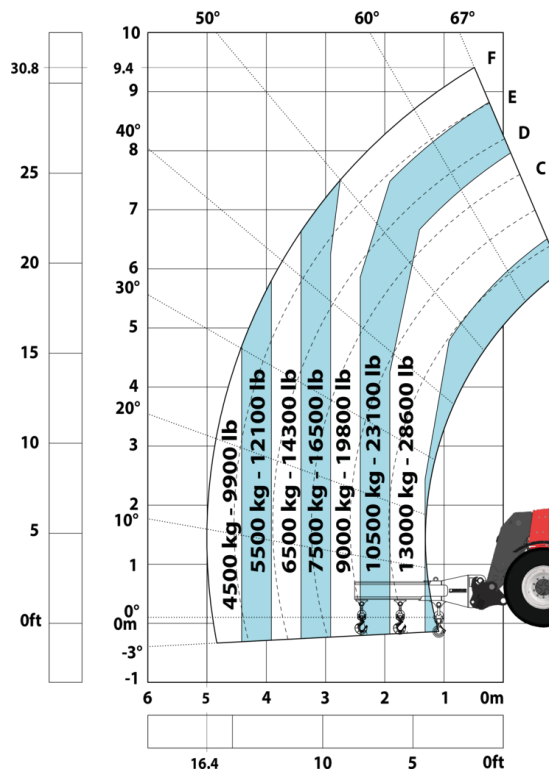
Machine on tyres with 3-hook jib 16000 kg (Metric)
